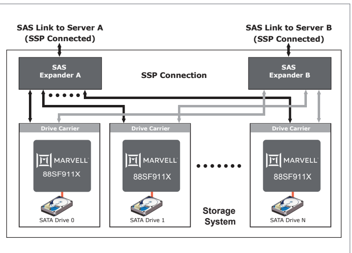
Figure 3. 88SF9110/9118 in Enterprise Storage System
