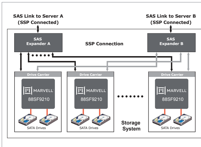
Figure 2. 88SF9210 in Enterprise Storage System
