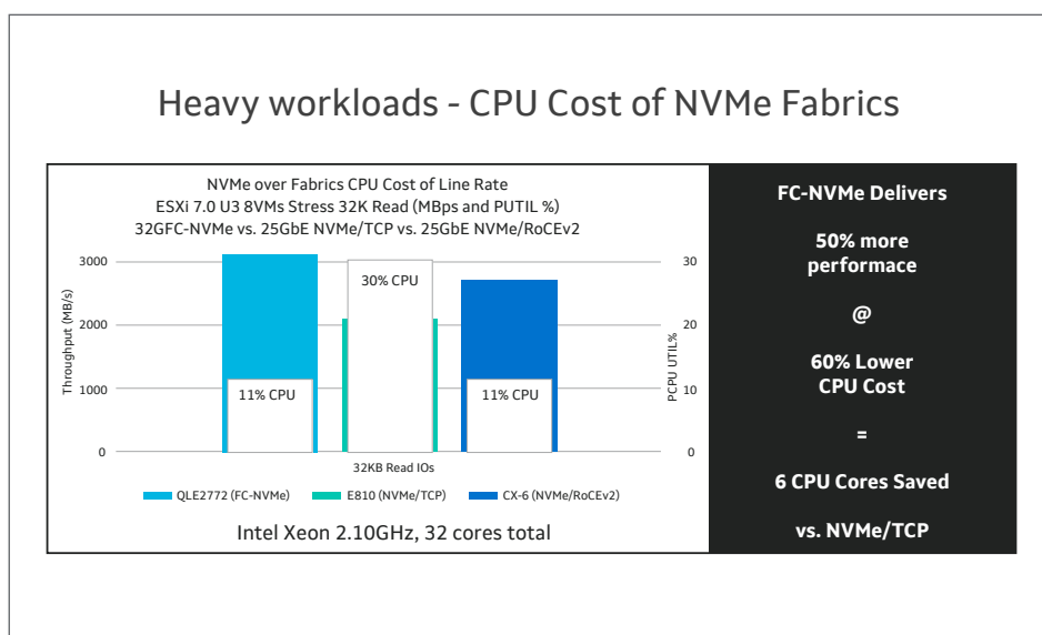
Figure 4: Heavy workloads - CPU Cost of NVMe Fabrics
